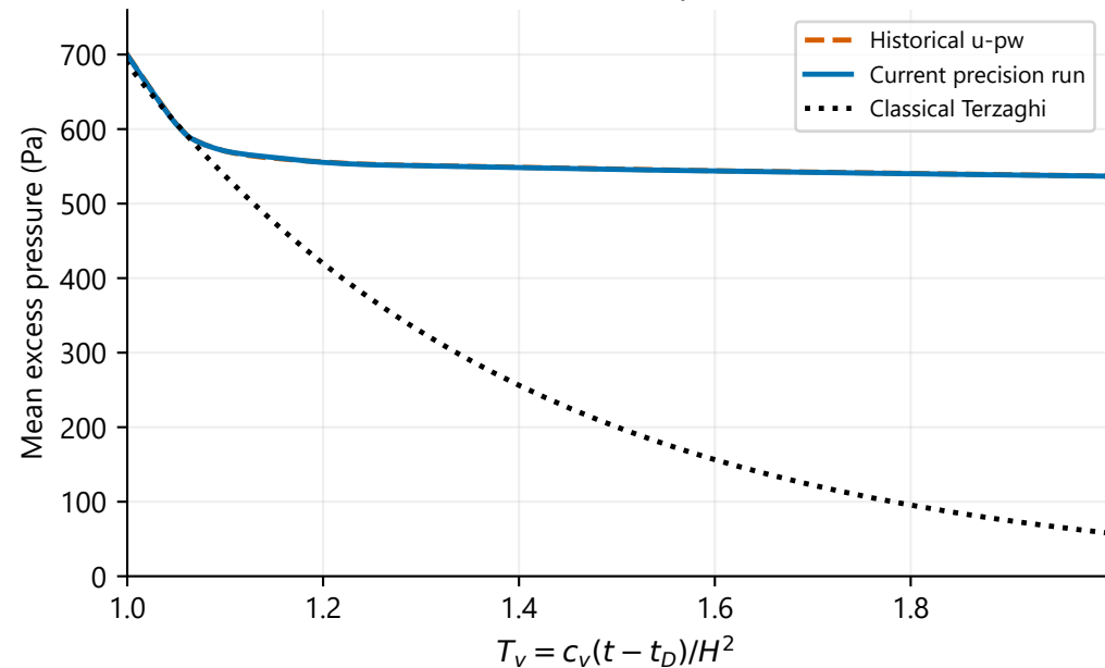
Late-time dissipation
