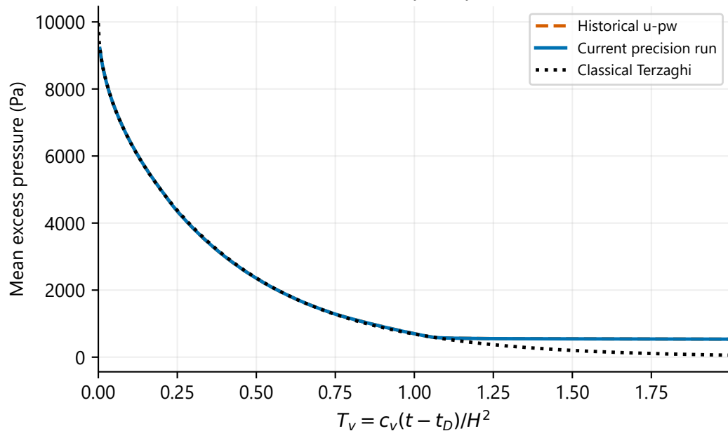
Mean excess pore pressure
