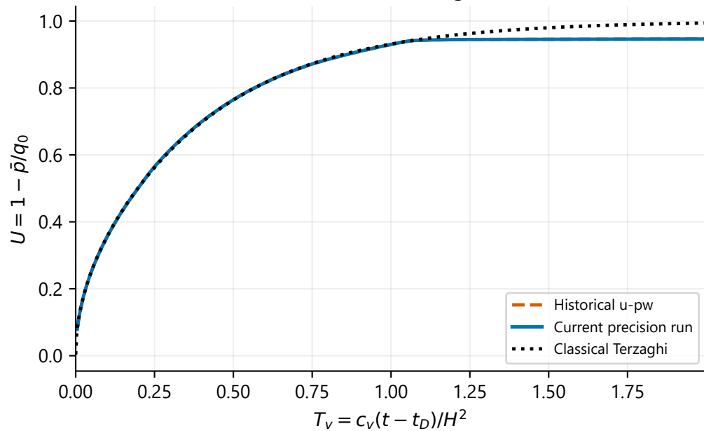
Consolidation degree
