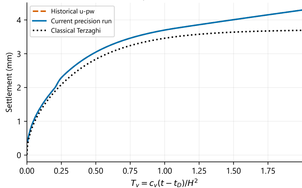
Top settlement
